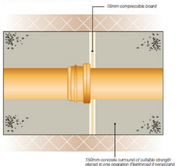
Figure 9: Pipe Protection – concrete surround
