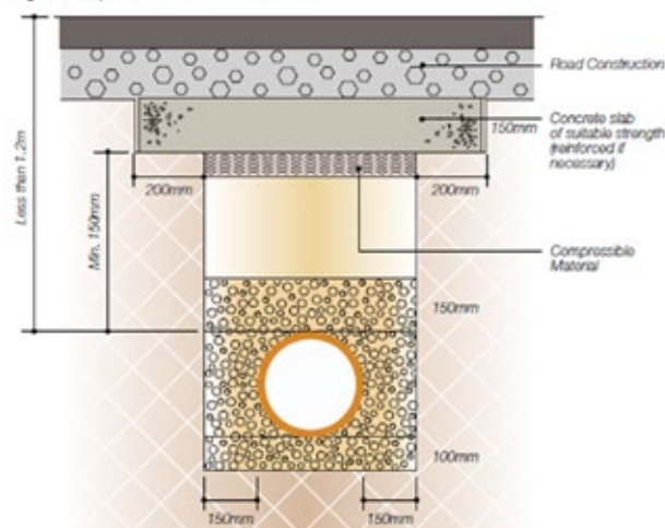
Figure 9: Pipe Protection – concrete surround
