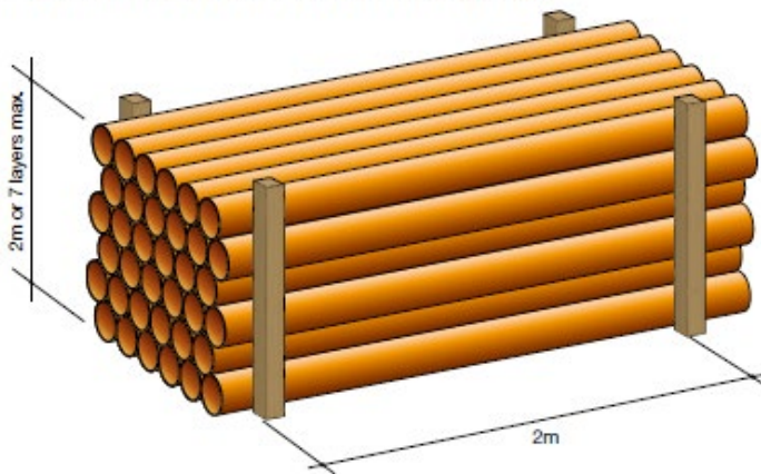
Figure 2: Storage of loose pipes on the ground
