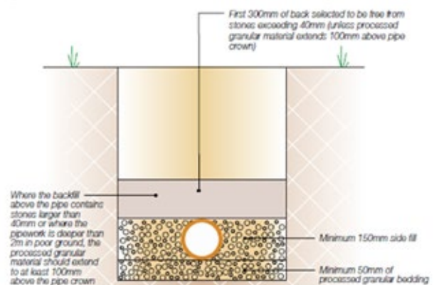
Figure 5: OsmaDrain pipes laid on 50mm minimum of processed granular material
