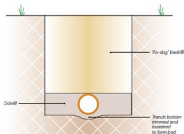
Figure 4: Hepworth Pipes laid on the trench bottom
