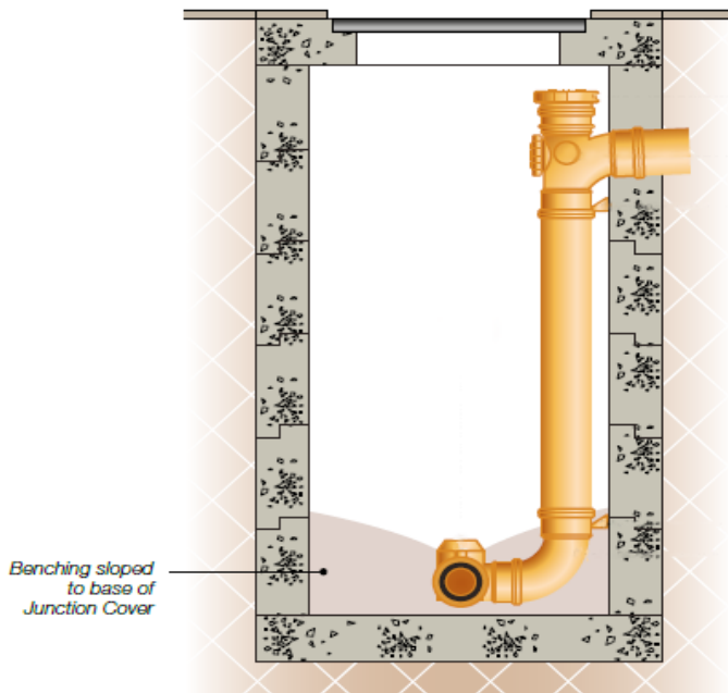
Figure 22: Sealed Access Manhole with internal backdrop
